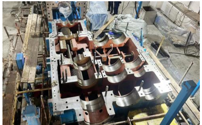
ZSK 320大型齿轮箱维修现场 Large gearbox ZSK 320 maintenance site
