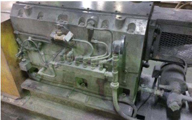
替换前的TEM-48SS齿轮箱 TEM-48SS gearbox before replacement
